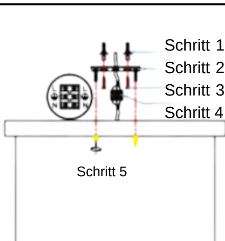
Installation Diagram
