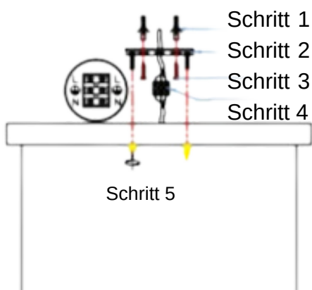
Installation Diagram
